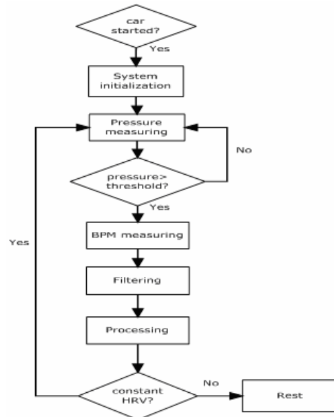
Fig. 4 Software's flow diagram
