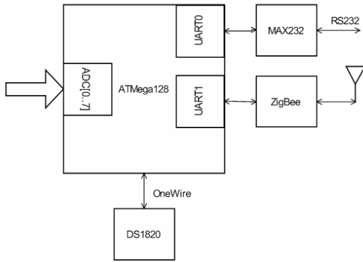
Fig. 2 Digital system. It is the one that receives the analogical signals, to digitize and process them. It also obtains temperature information and it has wireless communication capabilities.
